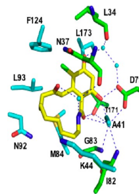
Figure 10. Hsp90-bound X-ray crystal structure of Moody's RAL macrolactam 121. 113 Image reprinted from ref 113. Copyright (2011) American Chemical Society.
