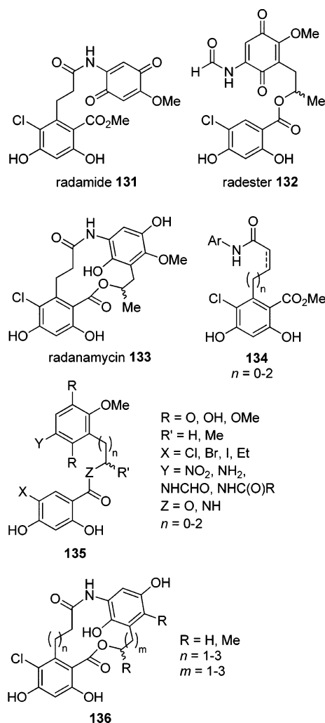
Figure 11. Blagg's radicol/geldanamycin "chimeras". 26,27,115–117
