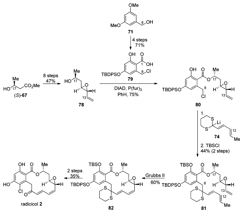
Scheme 14. Danishefsky's Total Synthesis of Radicol 2 (2001) 96
