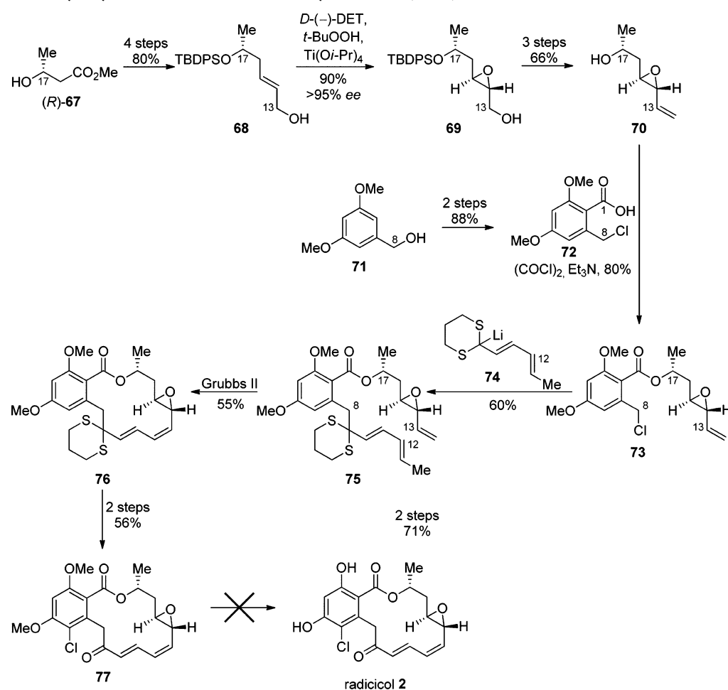
Scheme 13. Danishefsky's Synthesis of Radicol Dimethyl Ether 77 (2000) 101
